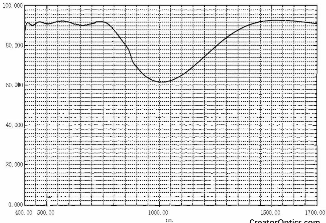
Transmittance of Sapphire Substrate with Dual-band Antireflection coating at 450 to 700nm and 1500nm to 1600nm
