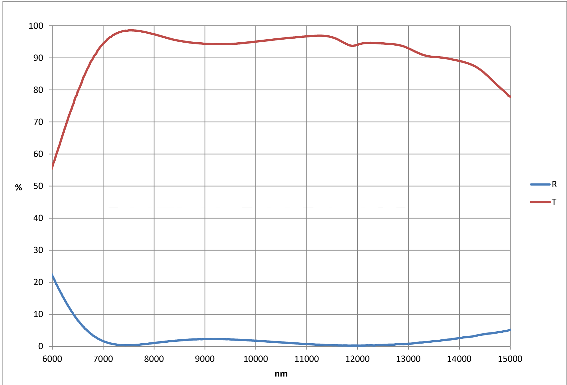
Transmittance and Reflectance of Anti-reflection coating at 7000 to 15000nm, 10.0mm thick germanium window, AOI=0°
