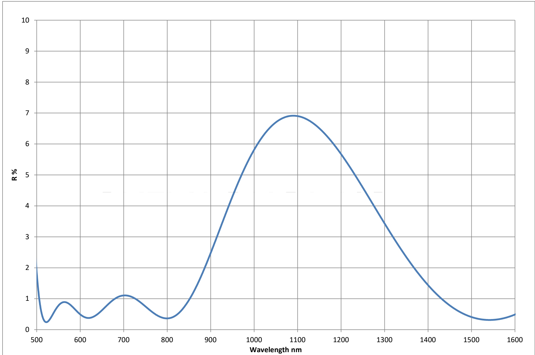
Reflectance of Dual Band Anti-reflection Coating, Fused Silica Window 2.0mm thick, AOI 0°
